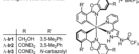
Scheme 1. Sources of chirality in asymmetric catalysts. See Ref. [6] ( \Lambda -Ir1) and the Supporting Information ( \Lambda -Ir2 and \Lambda -Ir3) for the synthesis of the enantiopure iridium catalysts. BARF 24 − = tetrakis[(3,5-di-trifluoromethyl)phenyl]borate.
